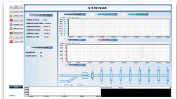
Statistics
